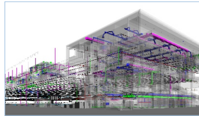
BIM MEPFP MODELING
