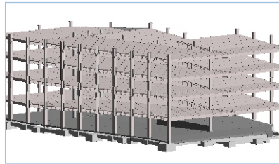
BIM STRUCTURAL MODELING
