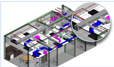
BIM COORDINATION AND CLASH DETECTION
